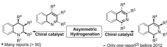
Scheme 1. Marked differences between the asymmetric hydrogenation of quinolines (left) and isoquinolines (right).
