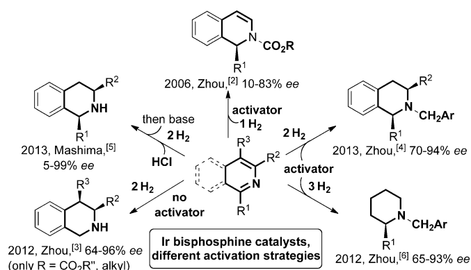
Scheme 2. Recent methods for the hydrogenation of substituted isoquinolines and isoquinolinium and pyridinium salts.
